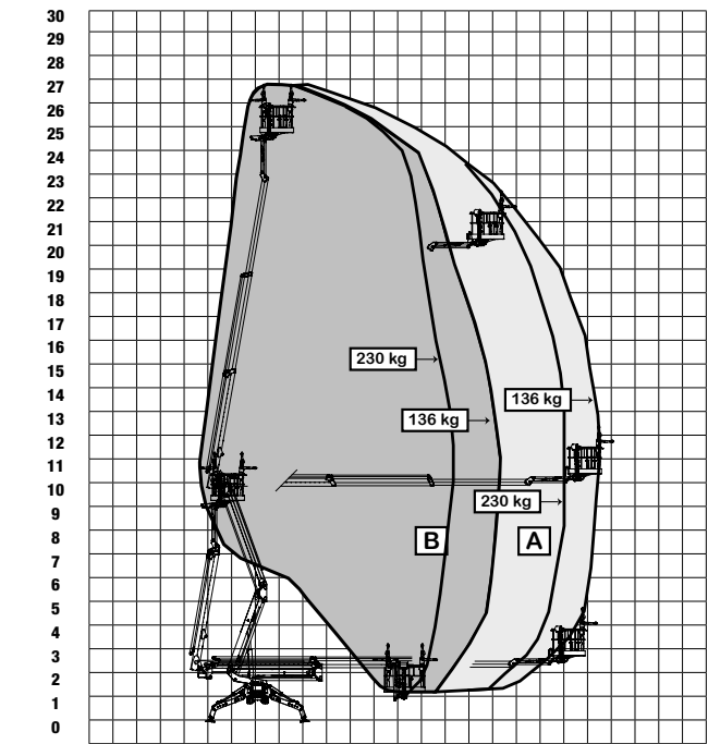
PLATFORM BASKET 27.14
