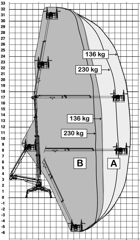
PLATFORM BASKET 33.15
