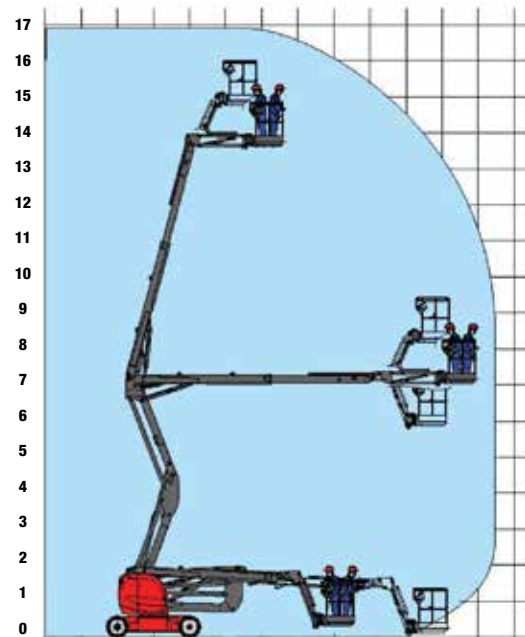
MANITOU 170 EATJ-L
